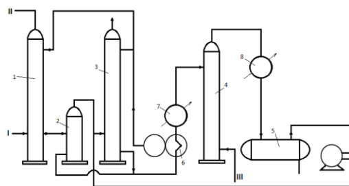
Fig.1. gas absorption facility by gas absorption is shown
